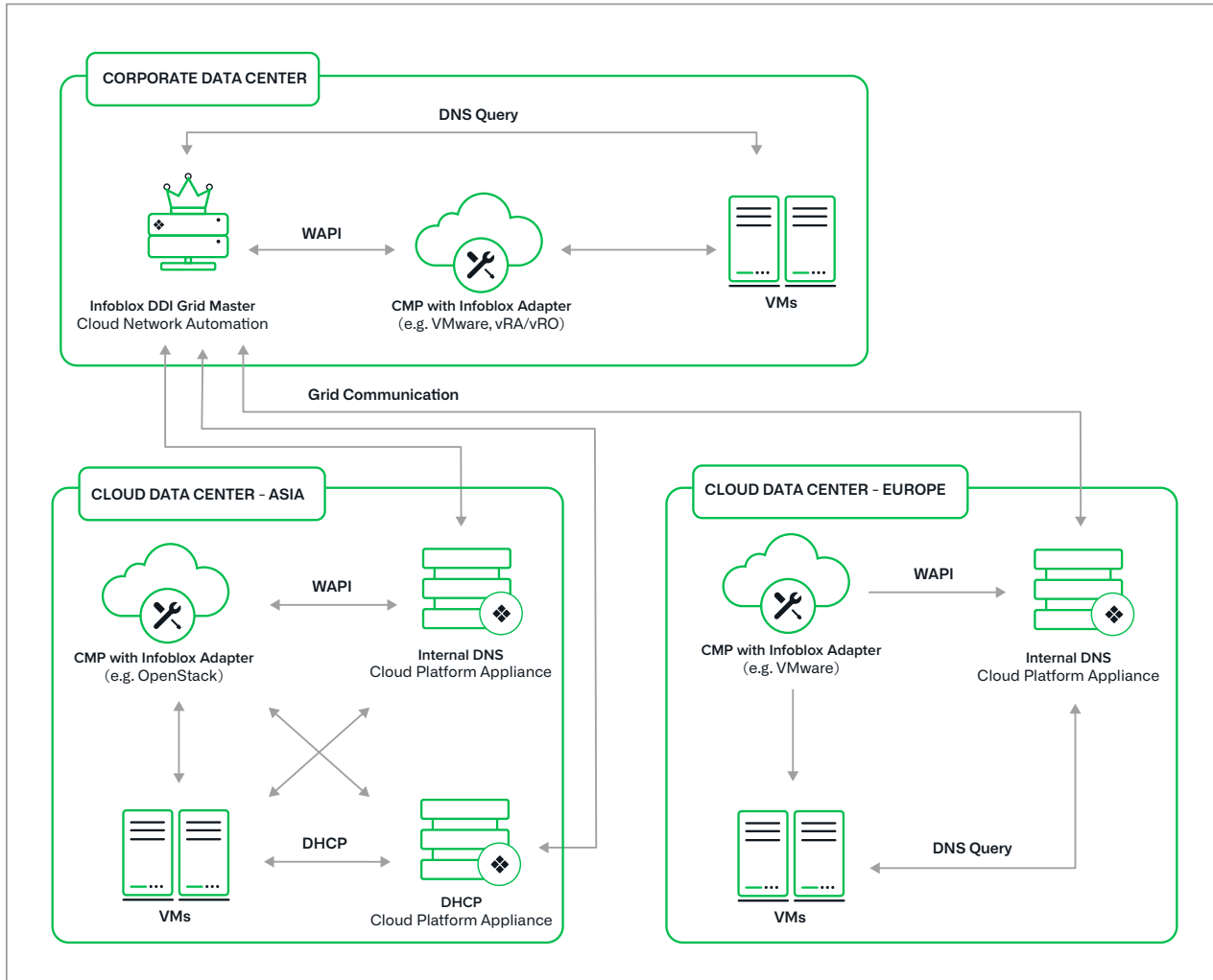
Figure 2: Sample deployment scenario using Cloud Platform Appliances with Infoblox DDI
